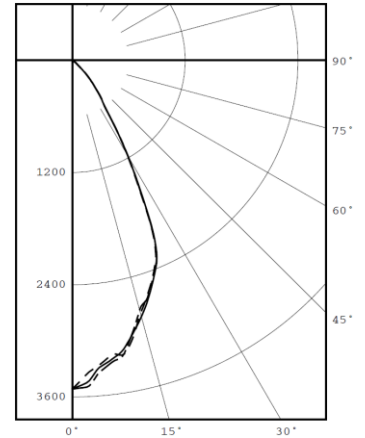
Candle Power Distribution
